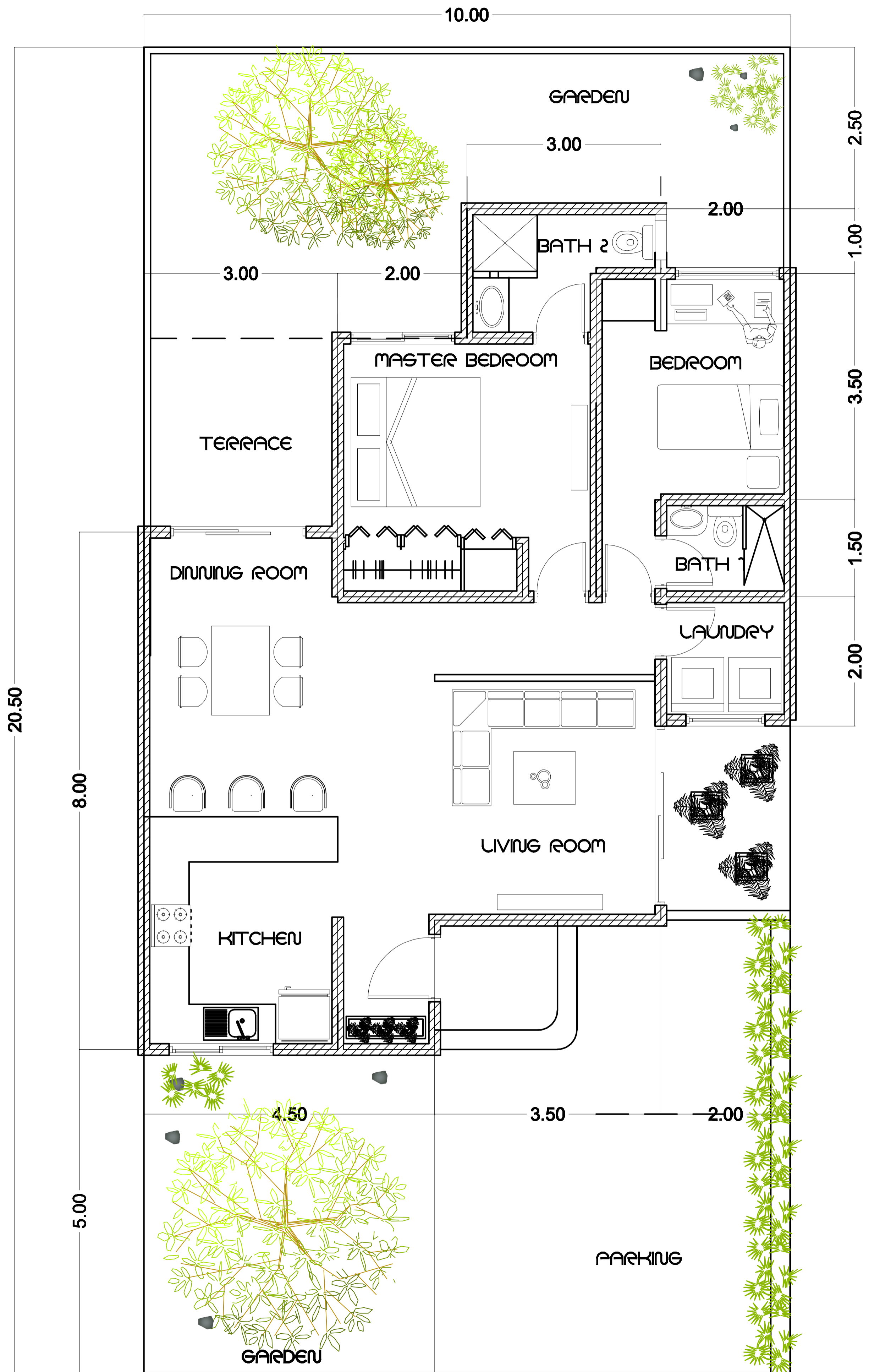
FLOOR PLAN
